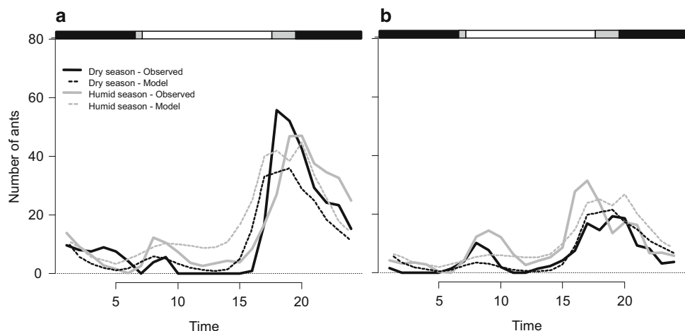
Fig. 2 Mean daily variation (observation and model) of the average number of ants observed per minute on a foraging trail for a Nest 1 and b Nest 2, for each hour of the day. The bar on the upper part of the graphic shows the time corresponding to the diurnal part (white rectangle) and the nocturnal part (black rectangle) of the nycthemere. The gray rectangles show the range of time in which sunrise or sunset occurs
